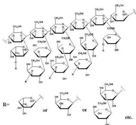
Chemical Structure of JUNSAI Polysaccharide
